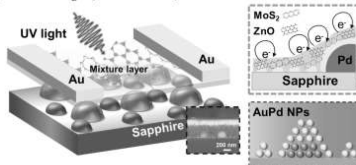
Figure 1: (a) Fabrication steps of hybrid \text{AuPd} nanoparticles (NPs) on sapphire (0001). (b) Side-view of hybrid UV photodetector (PD) incorporating \text{MoS}_2 nanoflakes (NFs), \text{ZnO} quantum dots (QDs) and hybrid \text{AuPd} NPs. [1]
