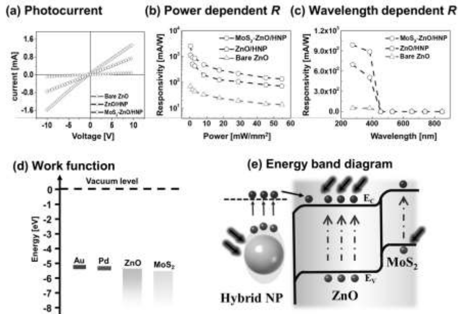
Figure 2: (a) – (c) Photoresponse for bare ZnO, ZnO/HNP and MoS 2 -ZnO/HNP PDs. (d) – (e) work function of various materials and energy band diagram. [1]
