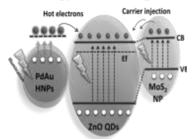
Figure 2. Morphological and optical characterization of hybrid PdAu NPs (a-1) SEM, (a-2) Extinction spectra, (a-3) FDTD simulation. (b) MoS 2 -ZnO/HNP PD (b-1) Photocurrent, (b-2) On/Off time, (b-3) Energy band diagram. [4]
